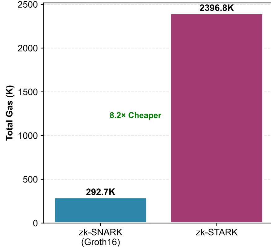
On-Chain Gas Cost
