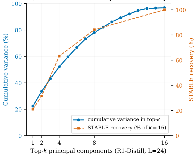
(B) R1-Distill's causal subspace is not the top-variance one
