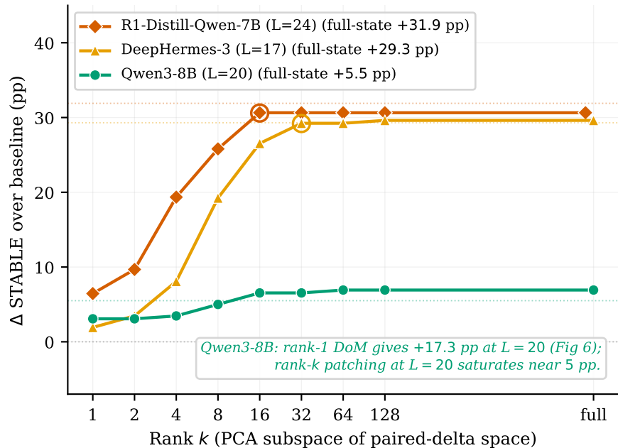
(A) Rank- k PCA patching: three reasoning models, three topologies
