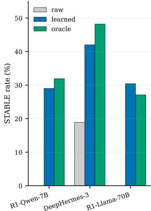
(C) Grounding before/after
