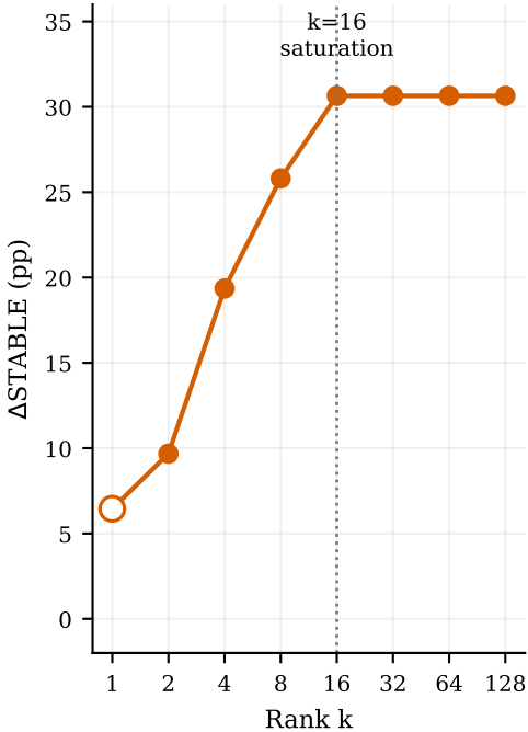
(A) Rank-1 is not enough
