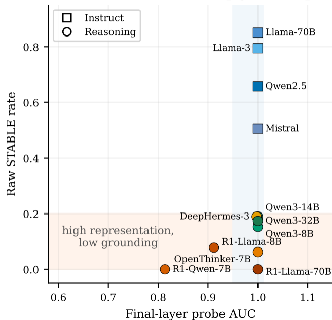
(B) Encoded does not imply acted upon
