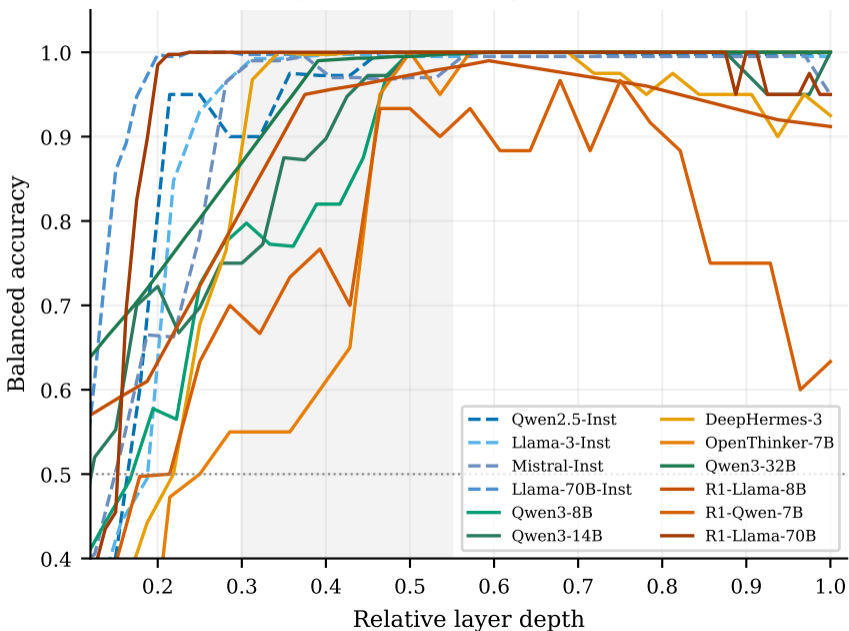
(A) Mismatch probe across layers
