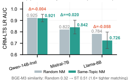
(a) Same-Topic Control (CRM-LTS)
