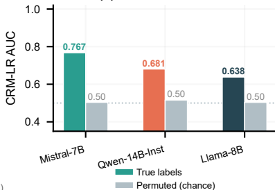
(b) Label Permutation
