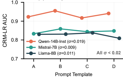
(c) Prompt Randomization
