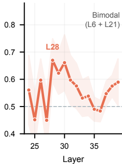
Qwen2.5-14B-Inst
