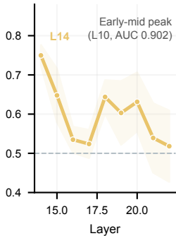
Qwen2.5-7B
