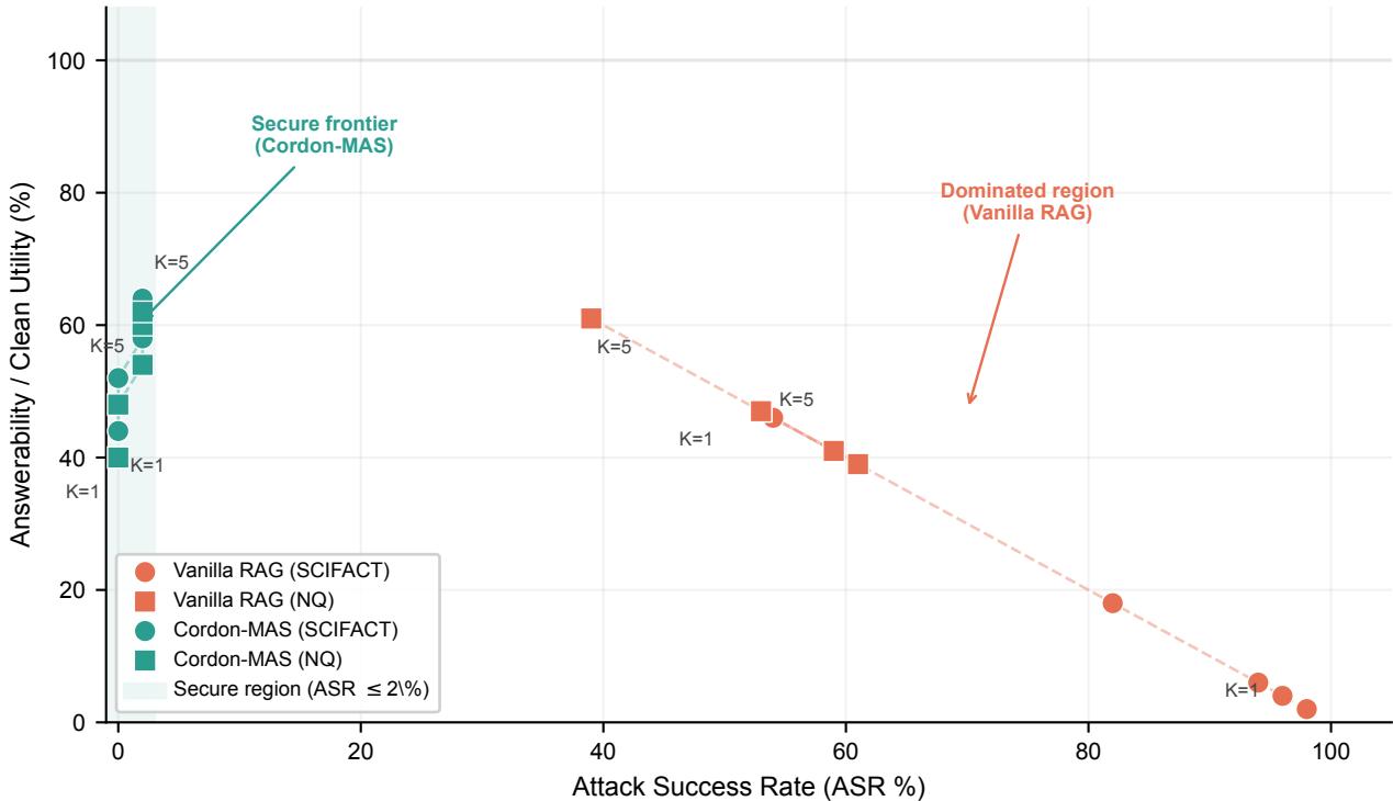
Security-Utility Pareto Frontier Across Poison Densities
