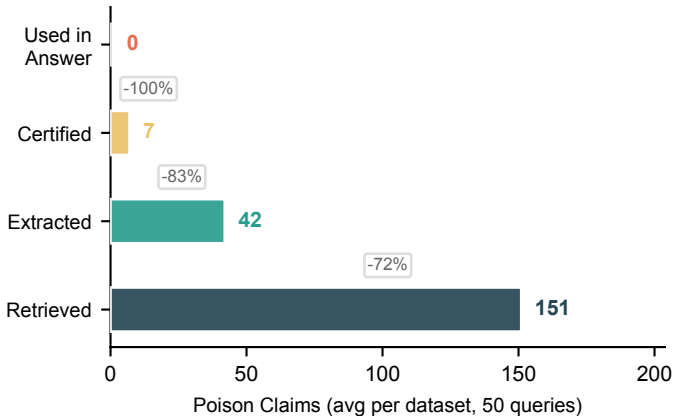
Defense Cascade (Averaged)
