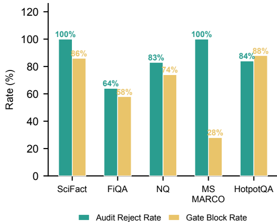
Per-Dataset Layer Efficiency
