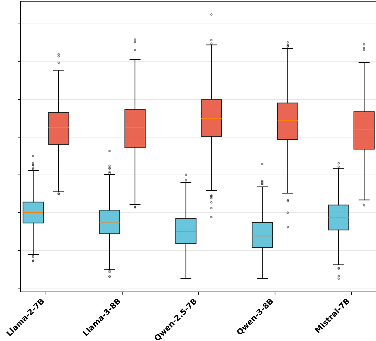
HotpotQA
