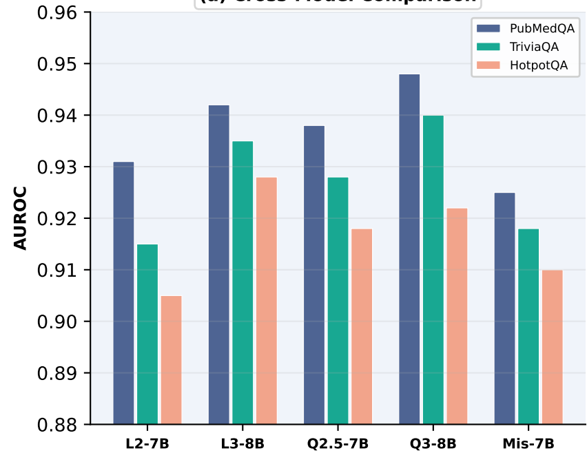
(a) Cross-Model Comparison
