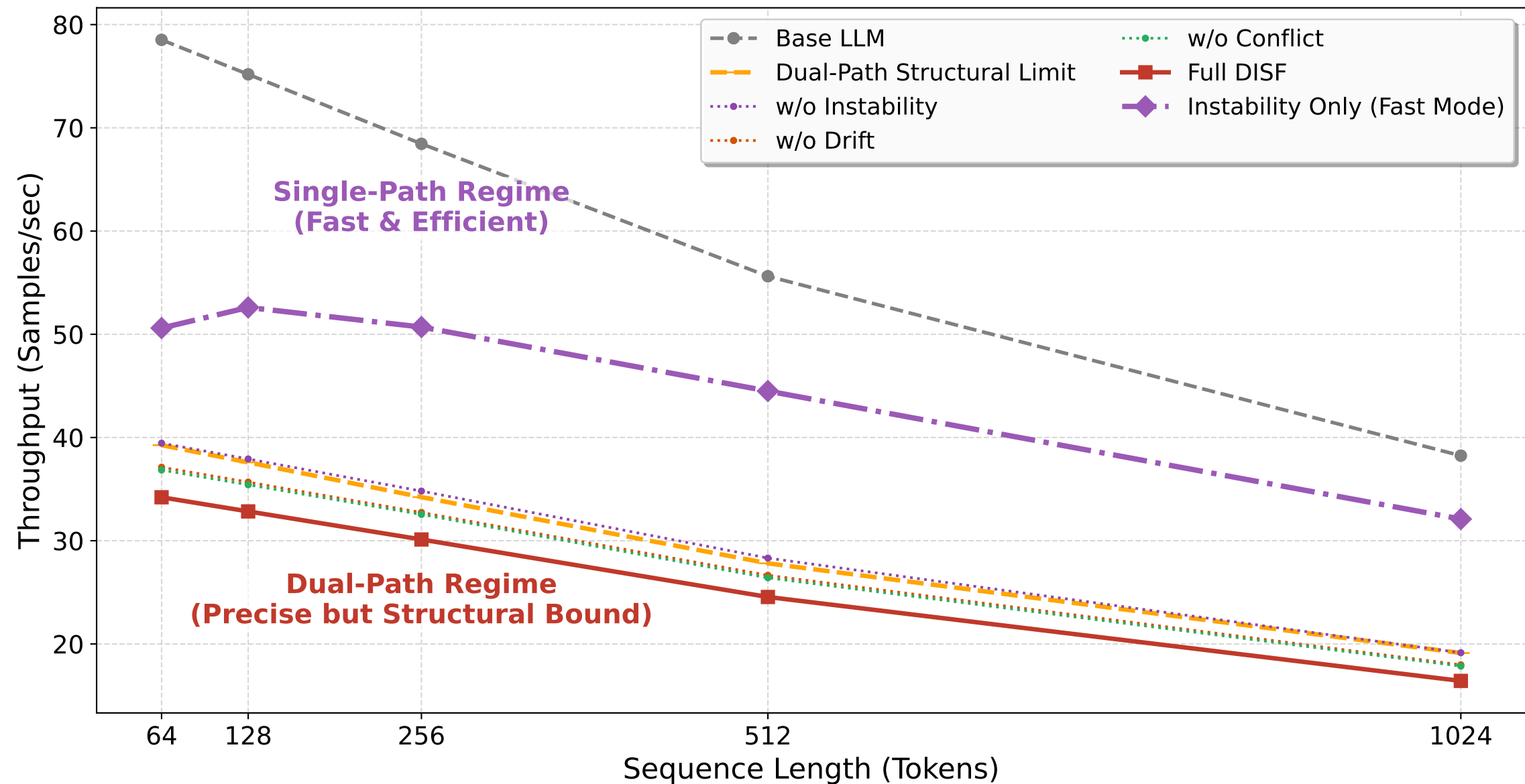
DISF Throughput: Structural Limits (Dual-Path) vs. Algorithmic Efficiency (Comprehensive Ablation Study)
