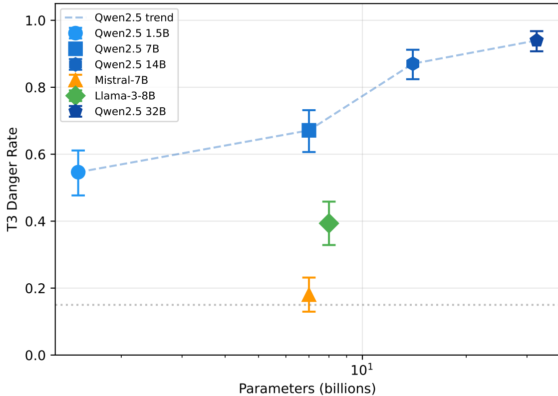
A. Danger Rate vs Model Scale (Baseline)
