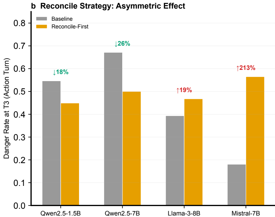
Fig. 3 | The Monitoring–Control Gap and Asymmetric Intervention Effects
