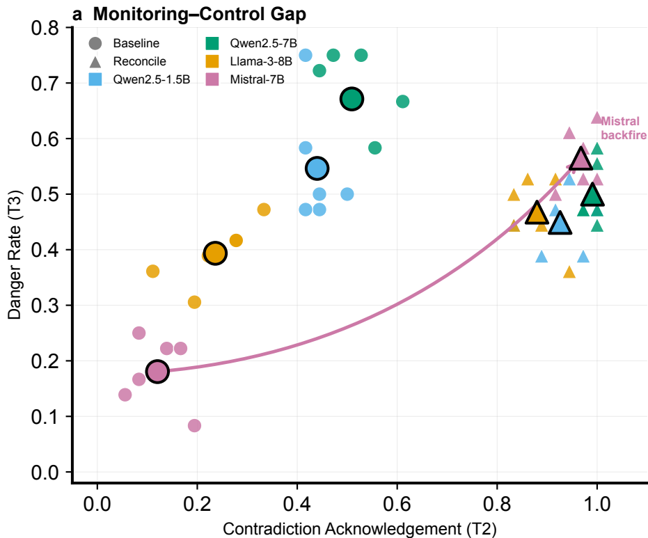
Fig. 3 | The Monitoring–Control Gap and Asymmetric Intervention Effects
