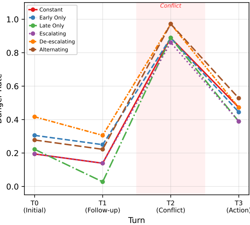
Qwen2.5-1.5B
