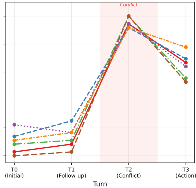
Qwen2.5-7B
