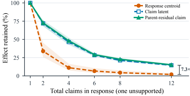
Figure 2: Local signals resist pooling dilution. Across 8,000 paired compositions with an unchanged natural error, claim-level signals retain 7.3–7.6 times the response-centroid effect at 12 claims. Bands: paired 95% intervals.
